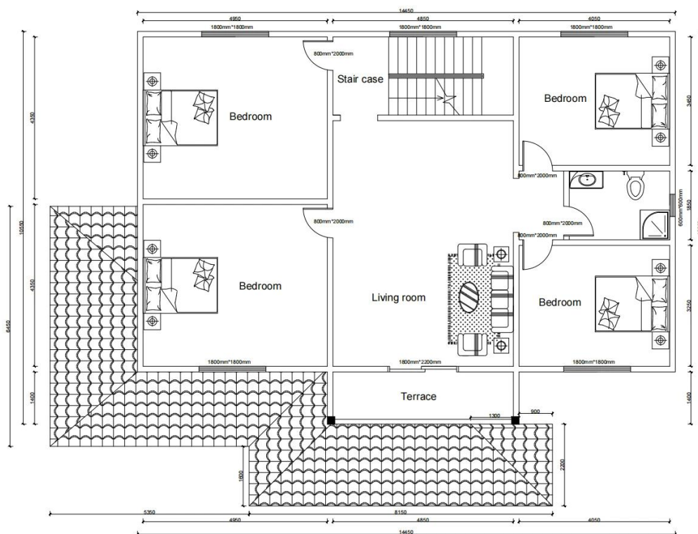
Second floor
