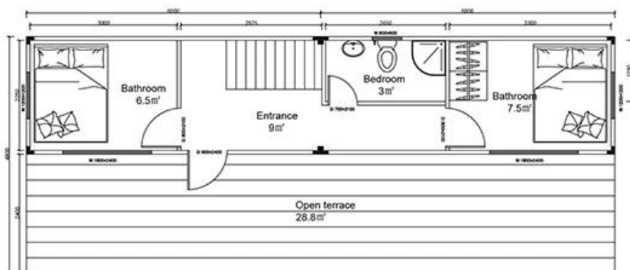
Second floor
