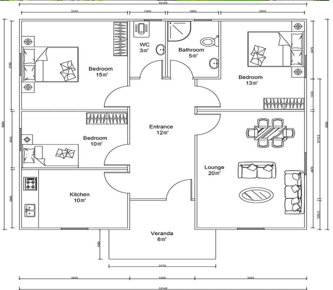
Prefab house details
