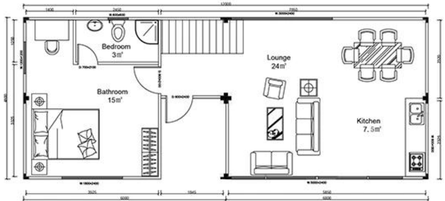
Ground floor
