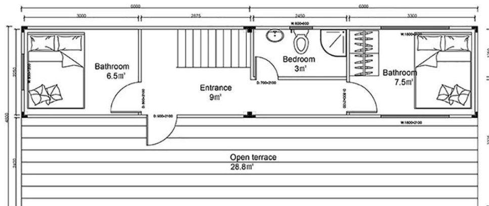
Second floor
